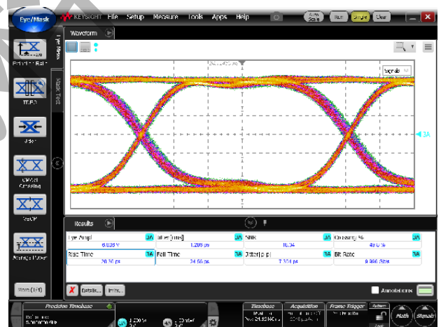
Data Rate = 10 Gb/s, V_{in} = 220 \text{ mV}_{pp}
